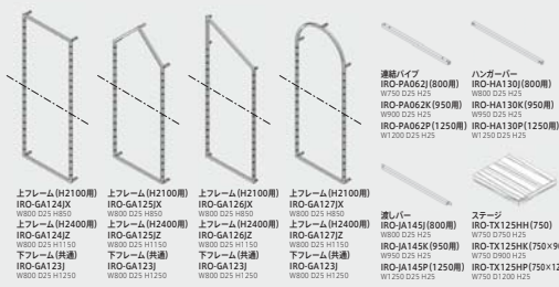
MODEL-43 W1250 D800 H2400
